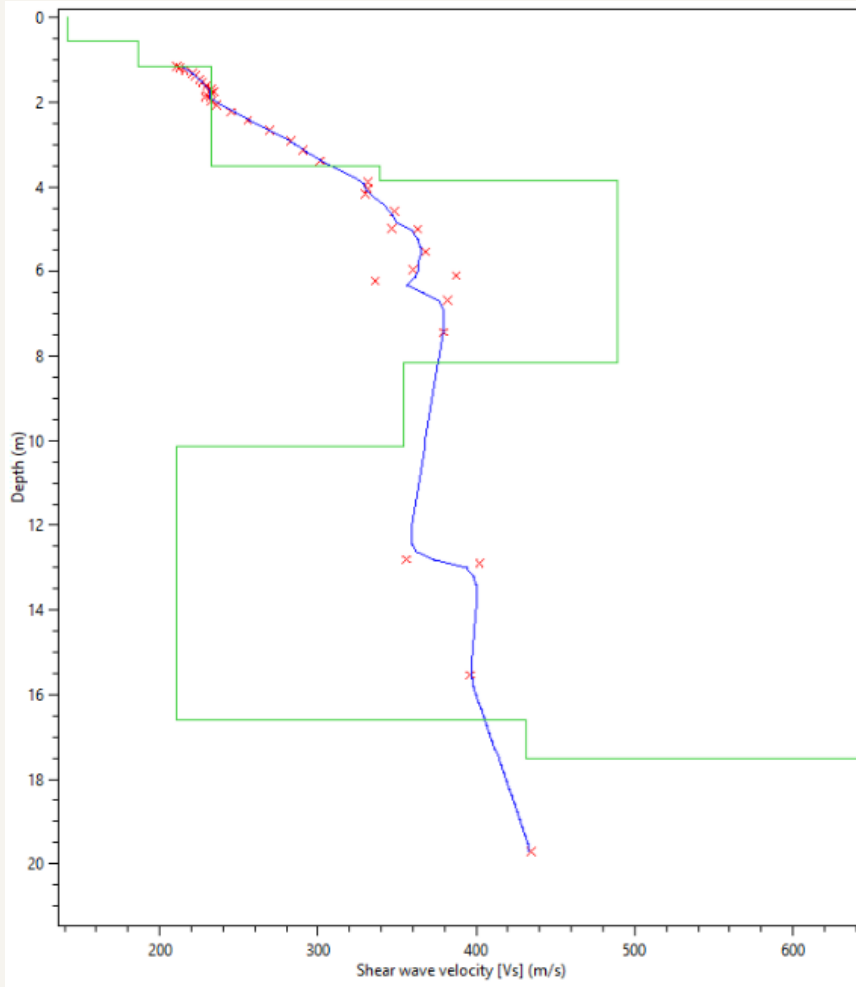
Figure 2: Low stiffness zone chalk in an area of collapsed mineworkings.
